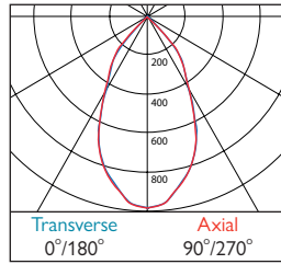
591 / 594 DLOR: 0.91 Chrome - Wide Beam
