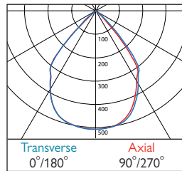
711/714 DLOR: 0.67 Dark Light - Wide Beam
