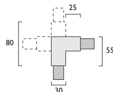
TS186A SCT 016 X Connector
